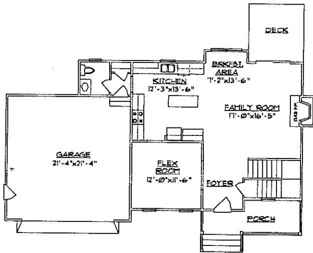
FIRST FLOOR PLAN 832 SQ. FT. (HEATED) 475 SQ. FT. (GARAGE)
