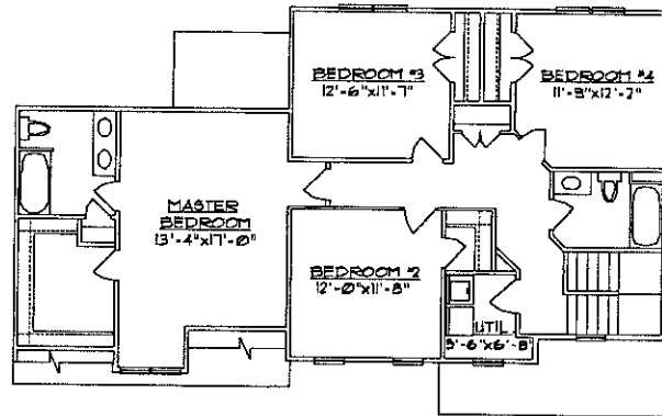
SECOND FLOOR PLAN 1235 SQ. FT. (HEATED)
