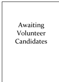
SERS Representative
