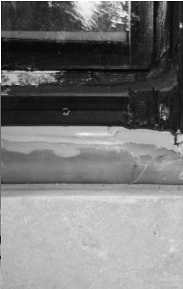
The Silicone Ribbed Extrusion is folded and sealed into the glazing pocket. Mechanical fasteners are used to hold the folded corner and are sealed over with Spectrem 1 Silicone Sealant.
