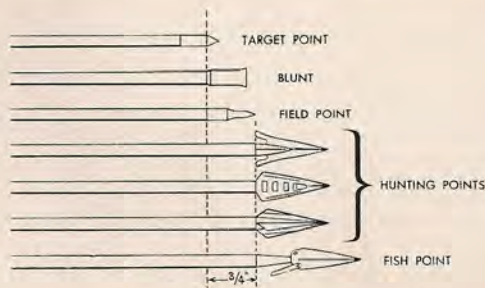
Arrow Length is Measured from Bottom of Nock to Point Indicated by Dotted Line
