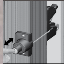
Optional Kit EXTERNAL ACCESS KIT Lockable Push-Button operates latch from outside the fence.
