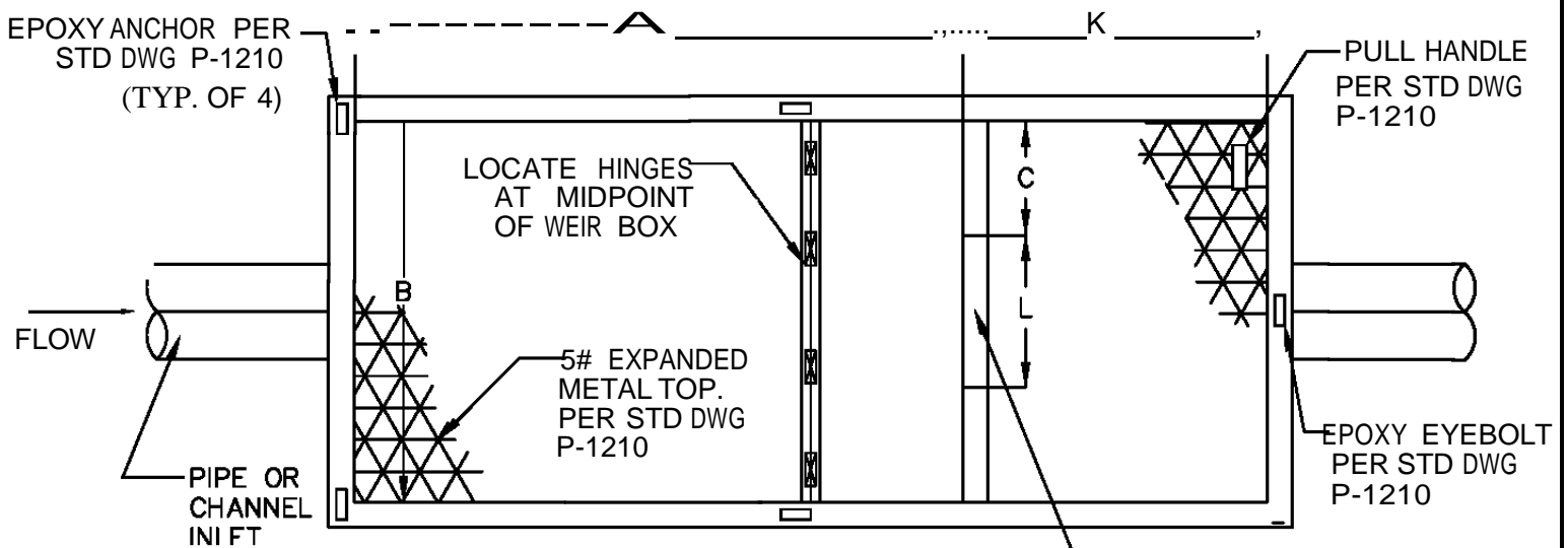
TOP VIEW
