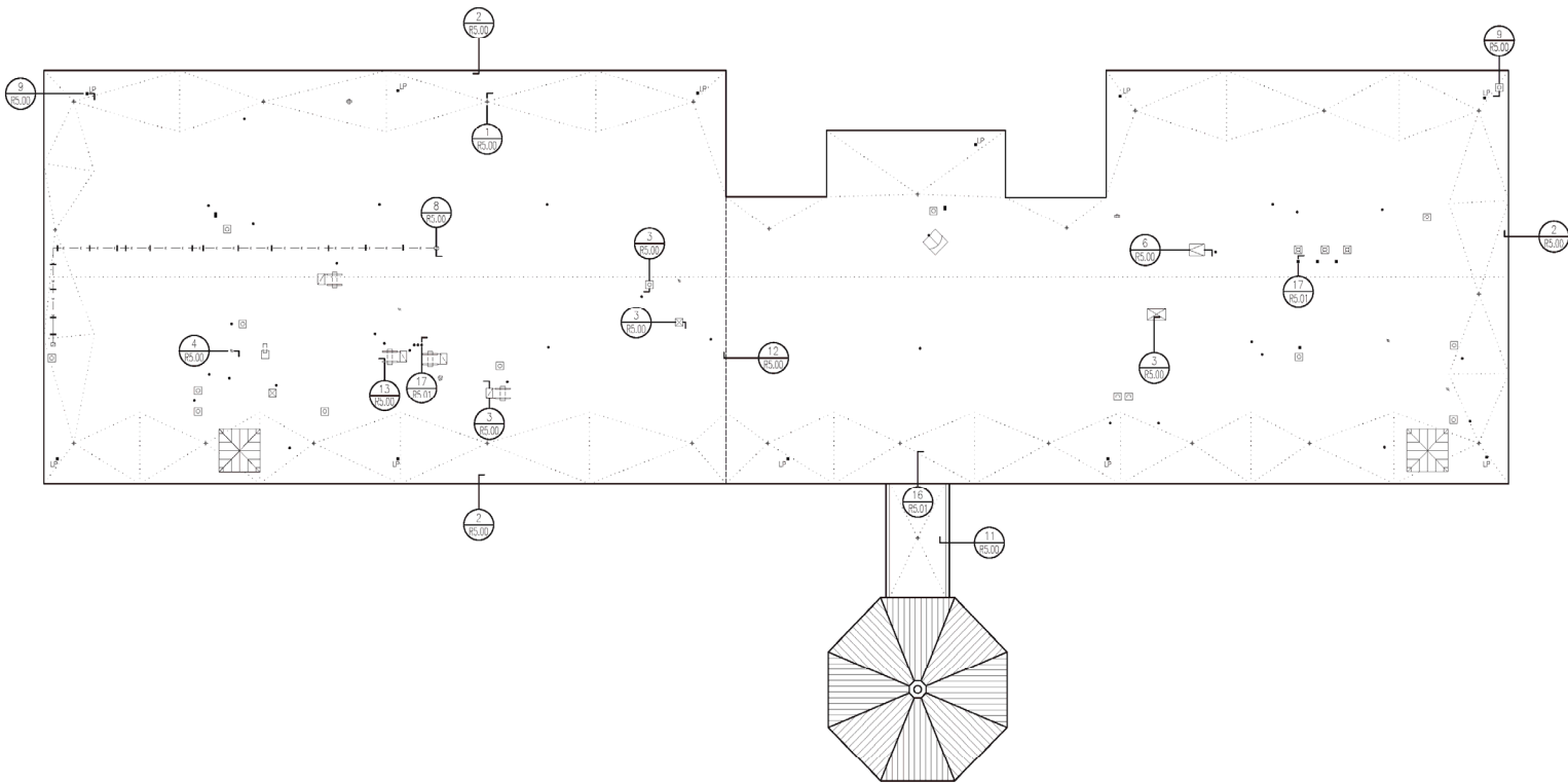
NEW ROOF PLAN: SCALE: 1/32"=1'-0" (11"x17"); 1/16"=1'-0" (22"x34")
