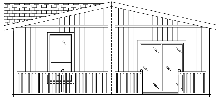
FRONT ENDWALL (W/OPT 8'-0" PORCH)
