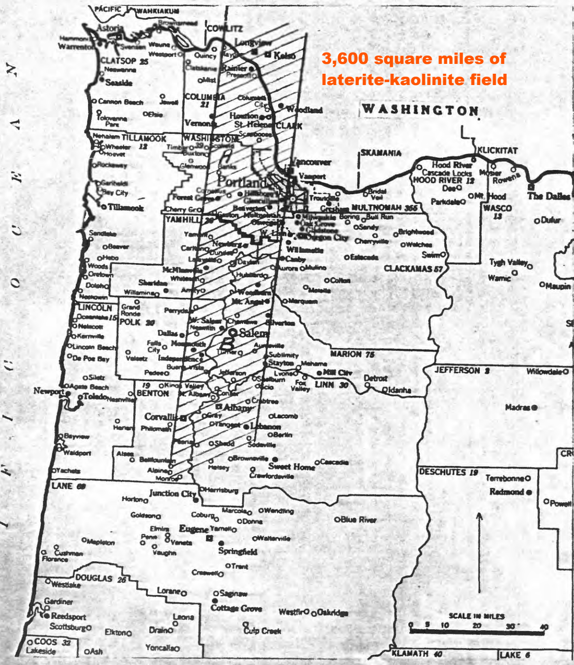
FIG. 1. - INDEX MAP OF NORTHWESTERN OREGON SHOWING BELT OF LATERITIC WEATHERING (Base map by Rand McNally)
