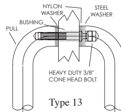
Type 13 Glass Door Back to Back
