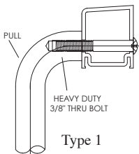
Type 1 Thru Bolt
