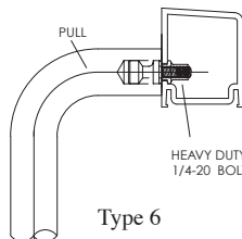
Type 6 Fully Concealed
