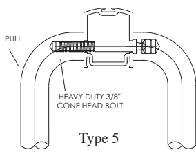
Type 5 Back to Back
