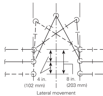
Horizontal Views
