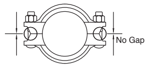
Metal-to-metal contact
