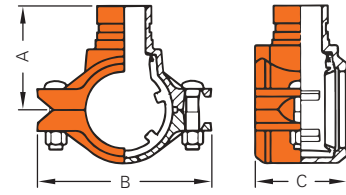
Grooved outlet
