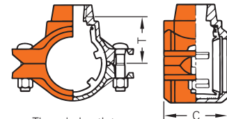
Threaded outlet
