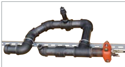
Burst pressure testing of DI threaded fittings (2')
