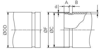
Figure 1 - Roll grooved-end dimensional reference points for Table 1
