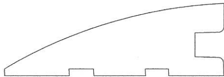
#8312 Clamshell 3/4" x 2-1/4"
