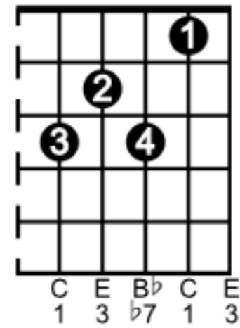
C 7
