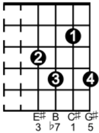
C# 7
