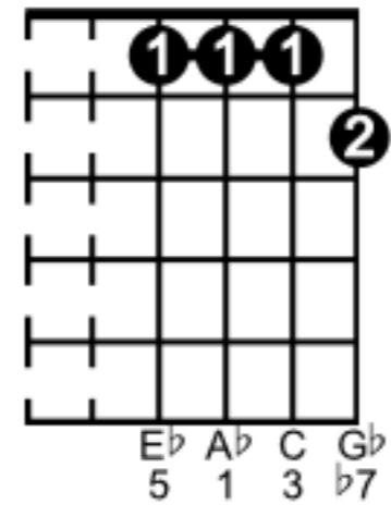
A \flat 7
