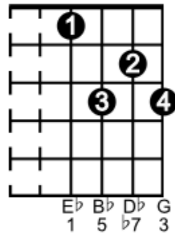
E \flat 7
