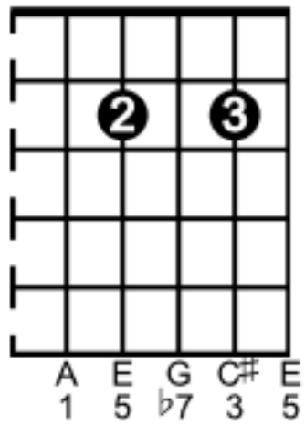
A 7
