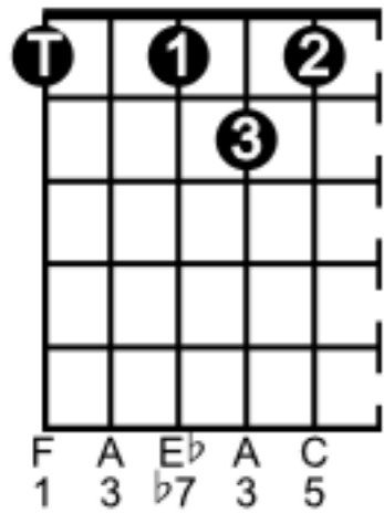
F 7
