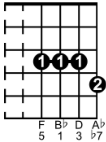
B \flat 7
