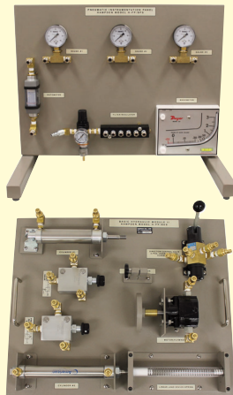
MODEL H-FP/BPS - H-FP/BHS Basic Pneumatics and Hydraulics Systems
