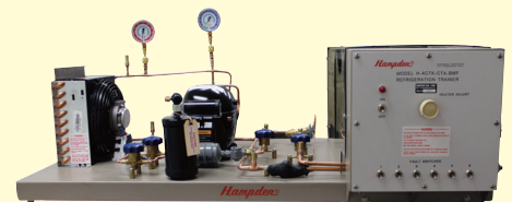
Model H-ACTK-CTA-BMF Refrigeration Trainer with Faults
