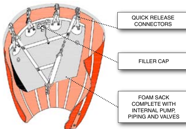
Sacksafoam™ I installed inside the Bambi Bucket®
