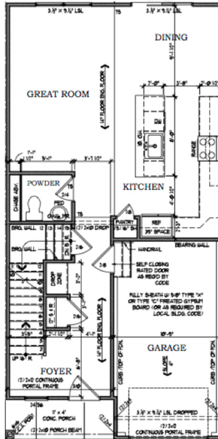
FIRST FLOOR
