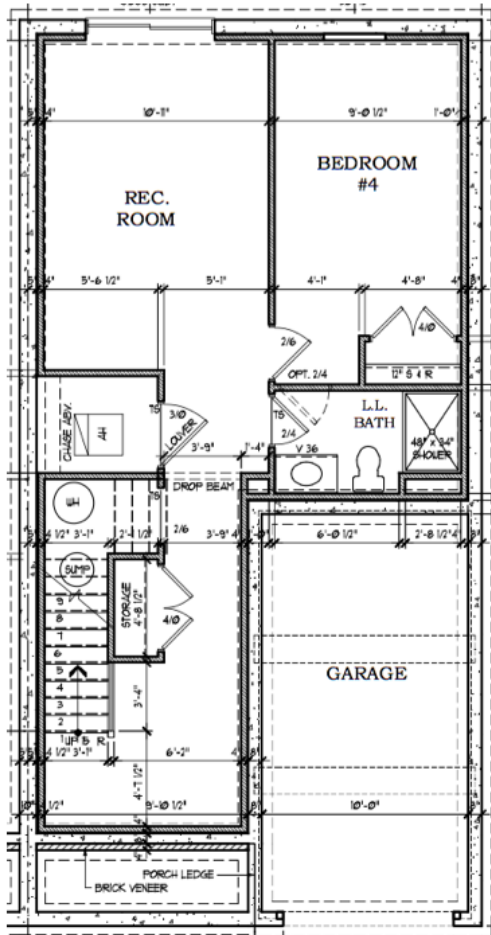
BASEMENT
