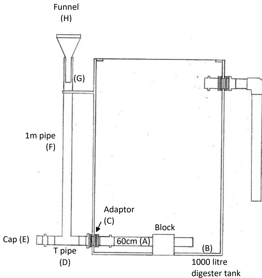
Figure 3-18: Assemble and fit the inlet pipe.
