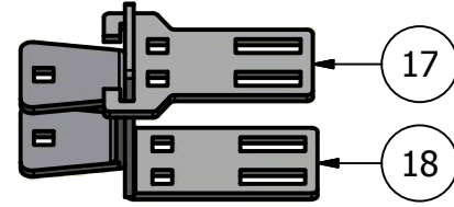
2" Multi-Bracket for the 1.75" Ext. Tube
