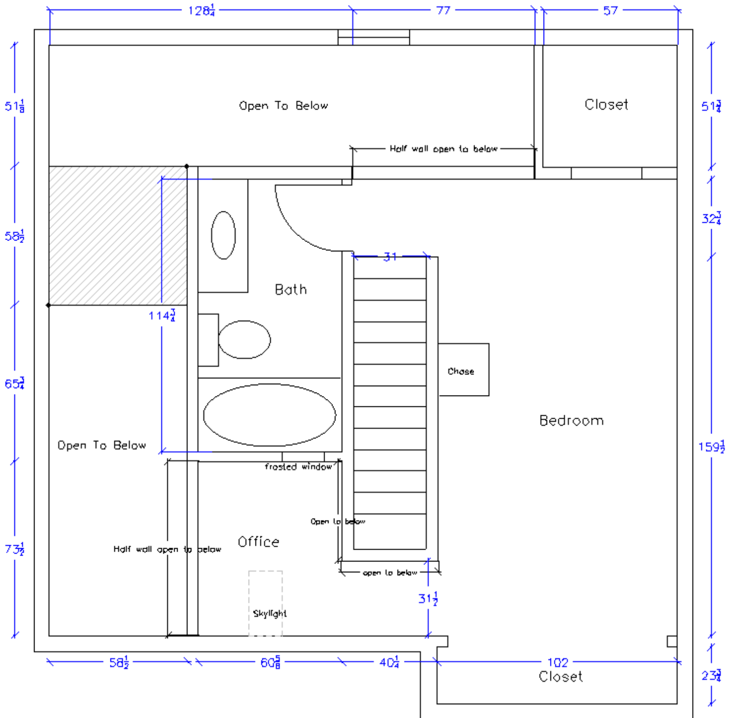
620 Pearl As-Built Upper Floor Not to Scale
