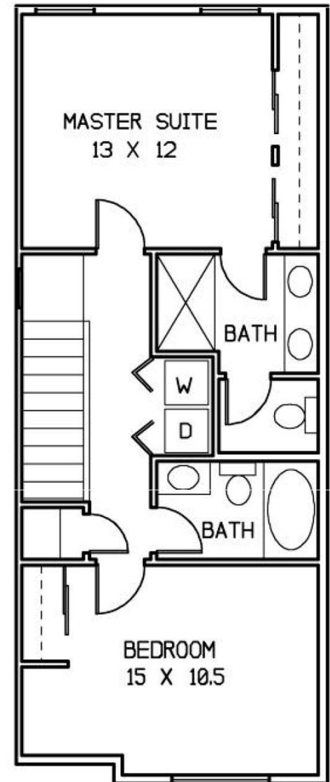
Second Floor
