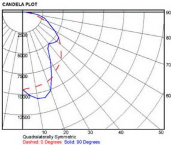
T5-6 Lamp IES File
