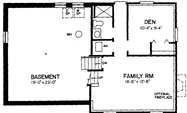
LOWER FLOOR PLAN (Four Bedroom Model)
