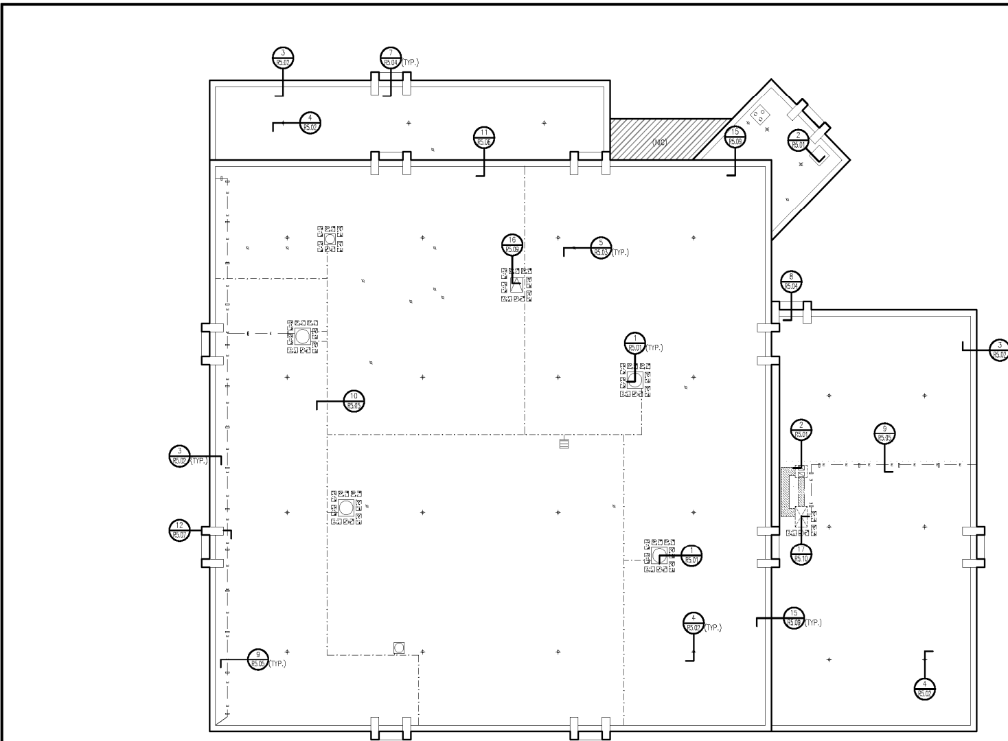
NEW ROOF PLAN: STARK MUSEUM OF ART SCALE: 1"=20'-0" (11'x17'); 1"=10'-0" (22'x34')
