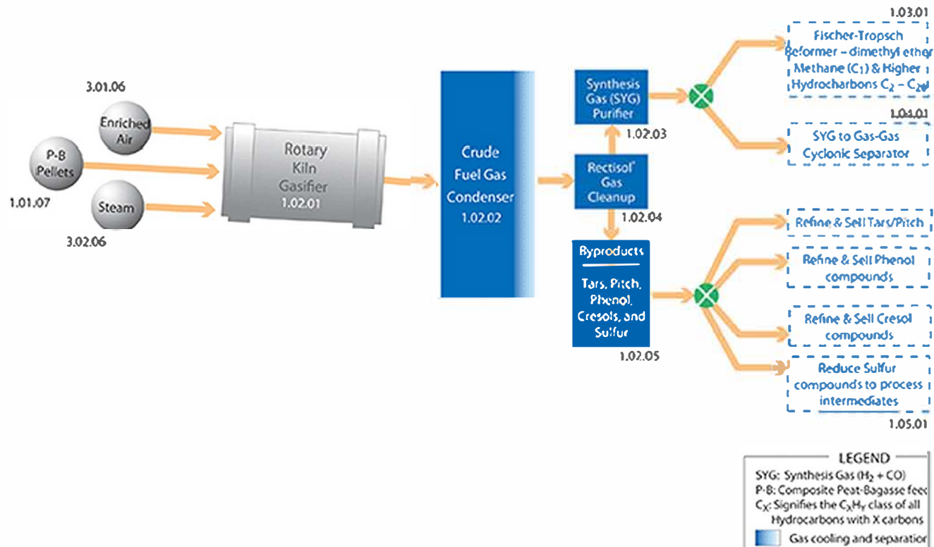
Peat-Bagasse Gasification Process
