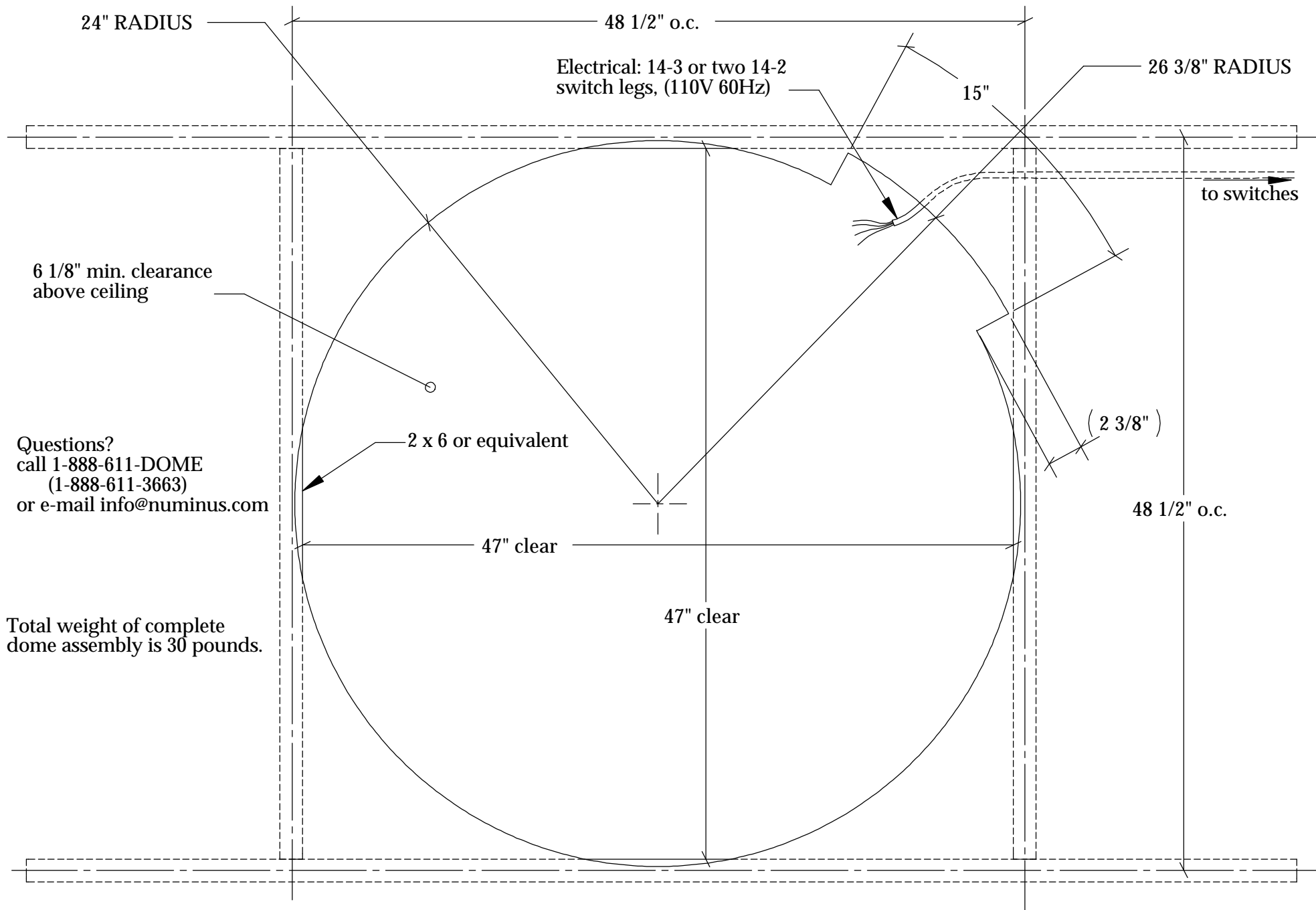
Rough-in drawing for flush mount installation of 4 ft Stardomes™ Architectural Starfield.
