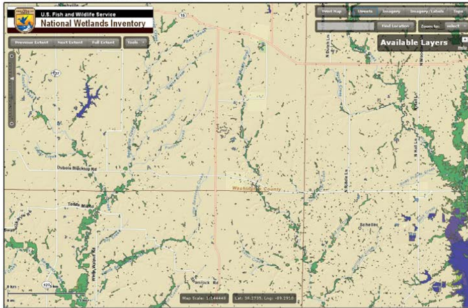
Figure 2–20. Examples of different landscapes showing interspersion of wetlands and streams or rivers (continued).
