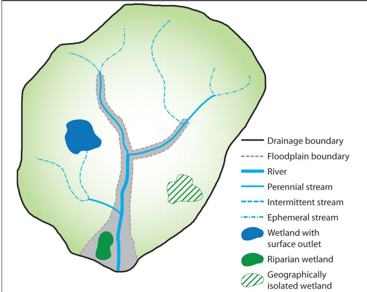
Figure 2-2. Elements of a river system. These elements include: the drainage basin (light green area), river network (rivers and streams), and other water bodies (riparian/floodplain wetlands, lakes, and wetlands in non-floodplain settings). Note that the non-floodplain wetland that lacks a stream outlet also would be considered “geographically isolated” sensu Tiner (2003b).
