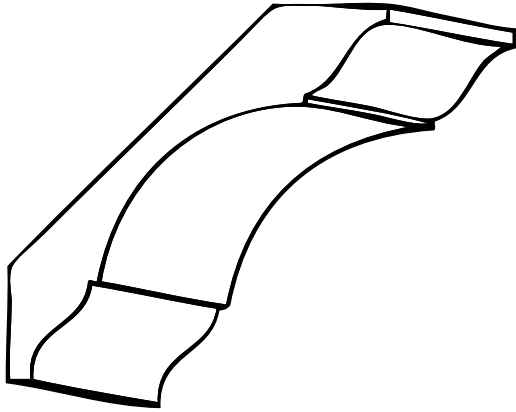
COVE PROFILE NO. : CR4001 PART NO. : T200 SIZE: 3/4" X 4"
