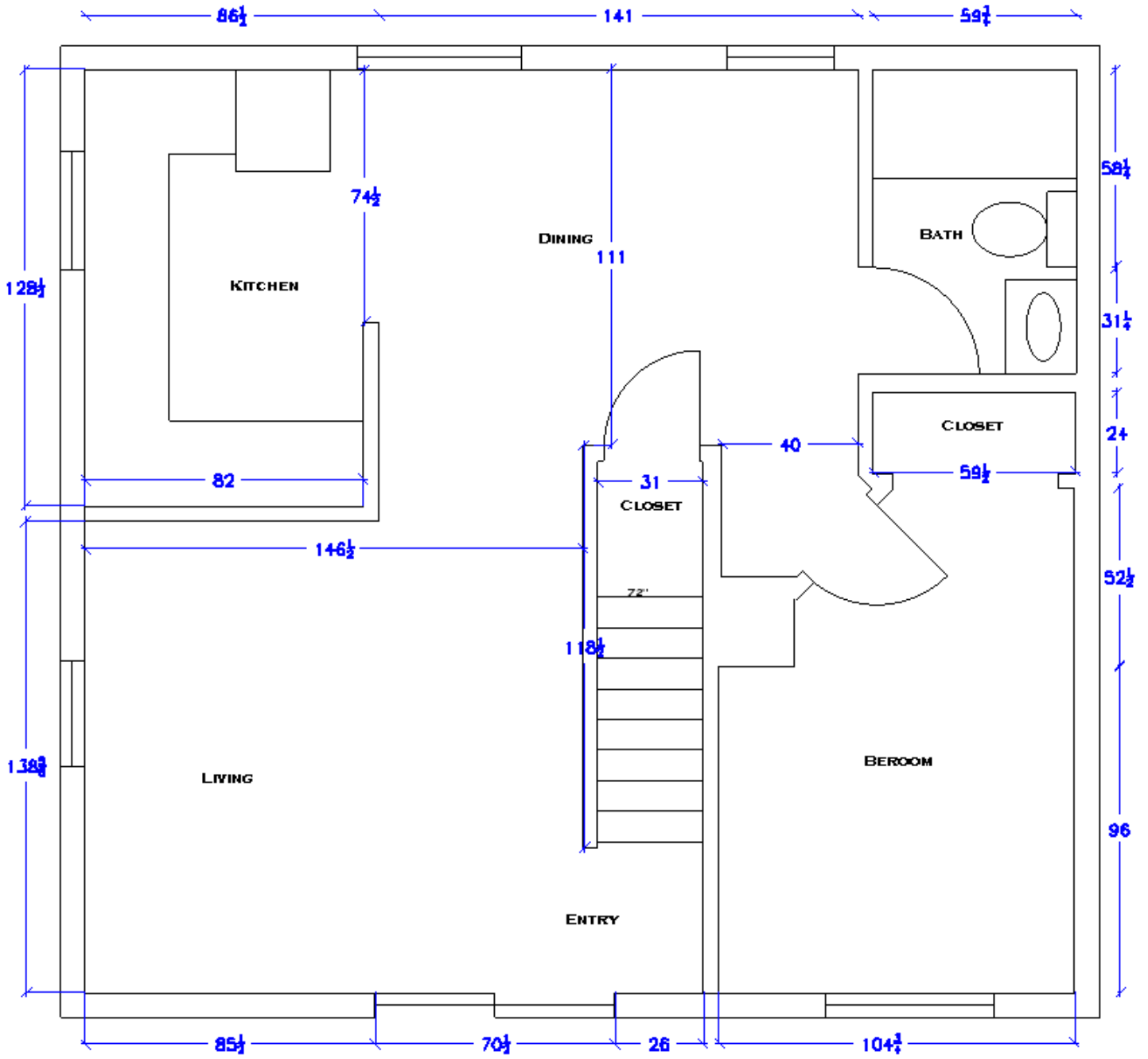
620 PEARL AS-BUILT LOWER FLOOR NOT TO SCALE
