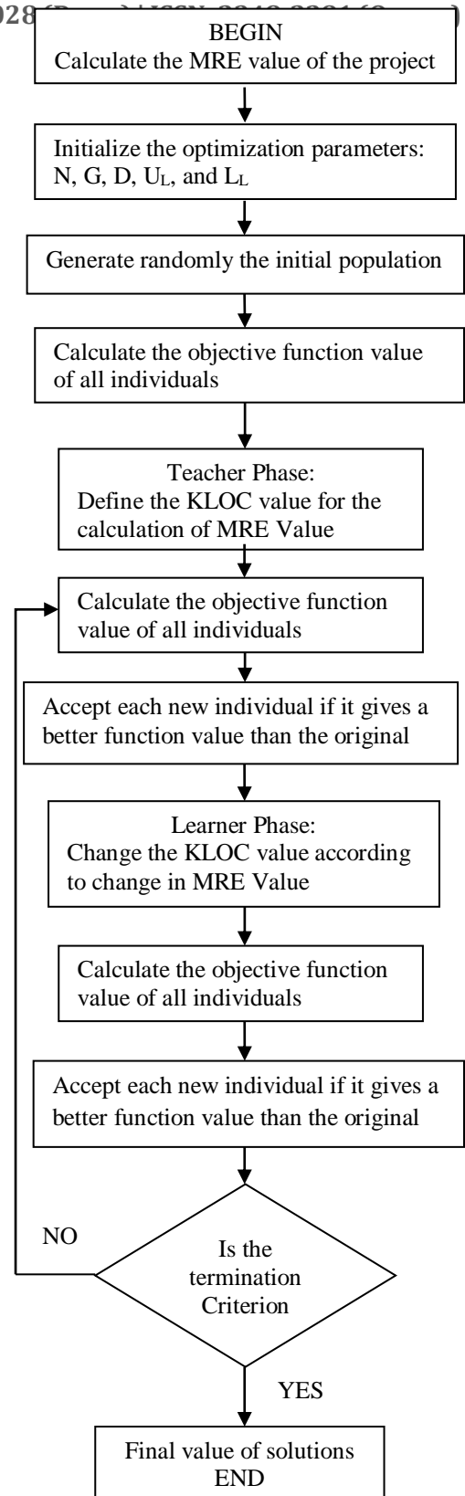
Figure 1: Proposed Flowchart
