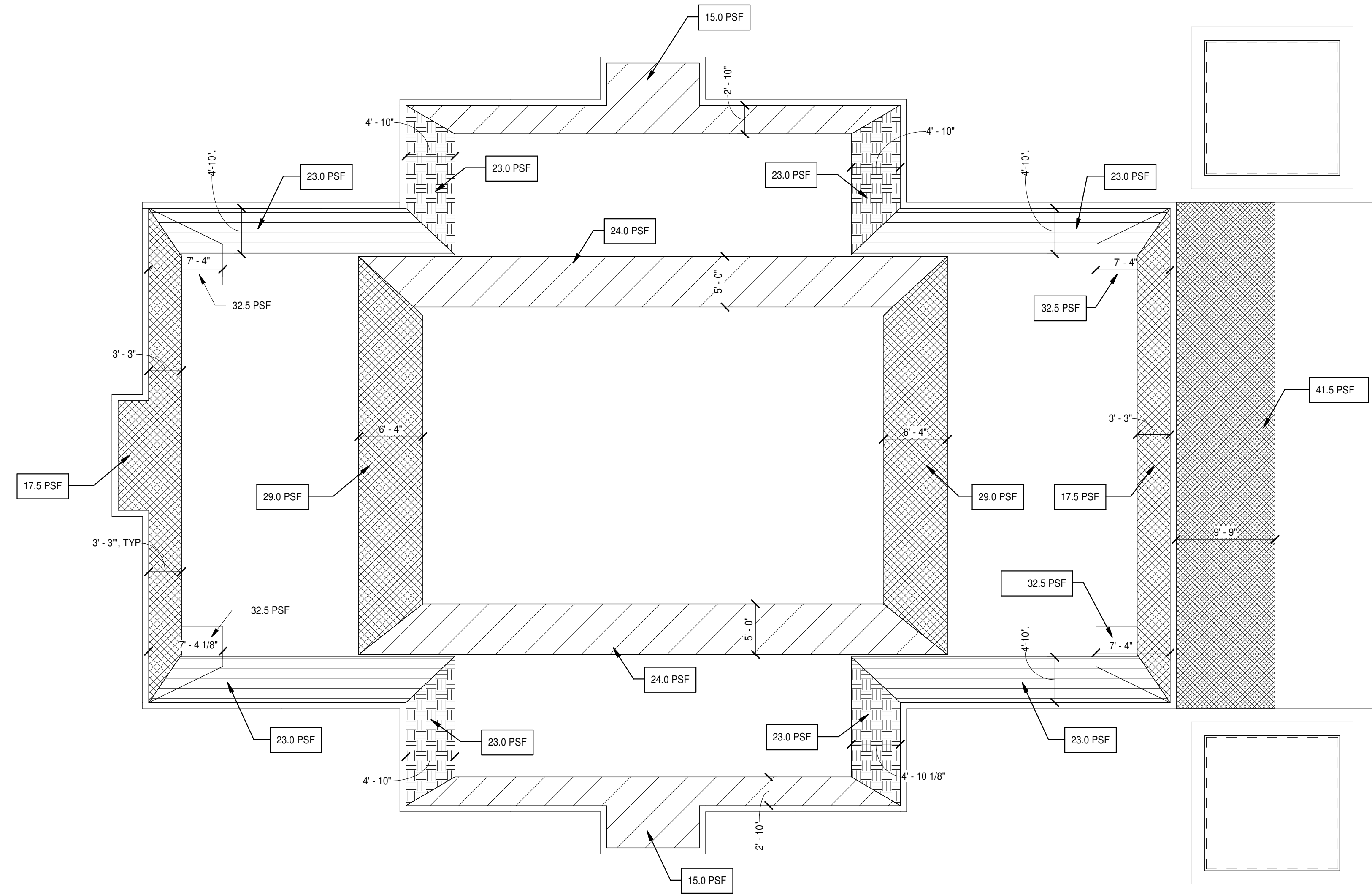
1 SNOW DRIFT LOAD DIAGRAM S3.0B 1/8" = 1'-0"
