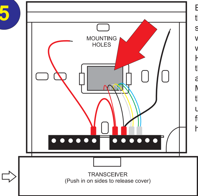
FRONT OF SUBBASE
