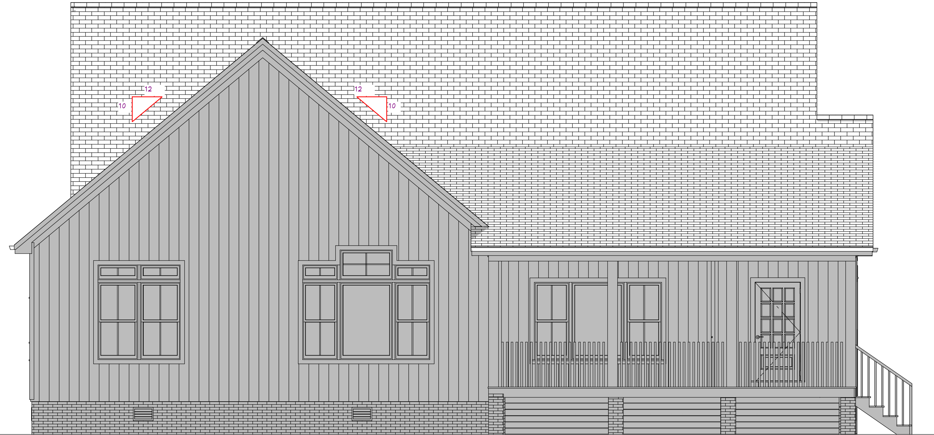
Exterior Elevation Back 1/4 in = 1 ft
