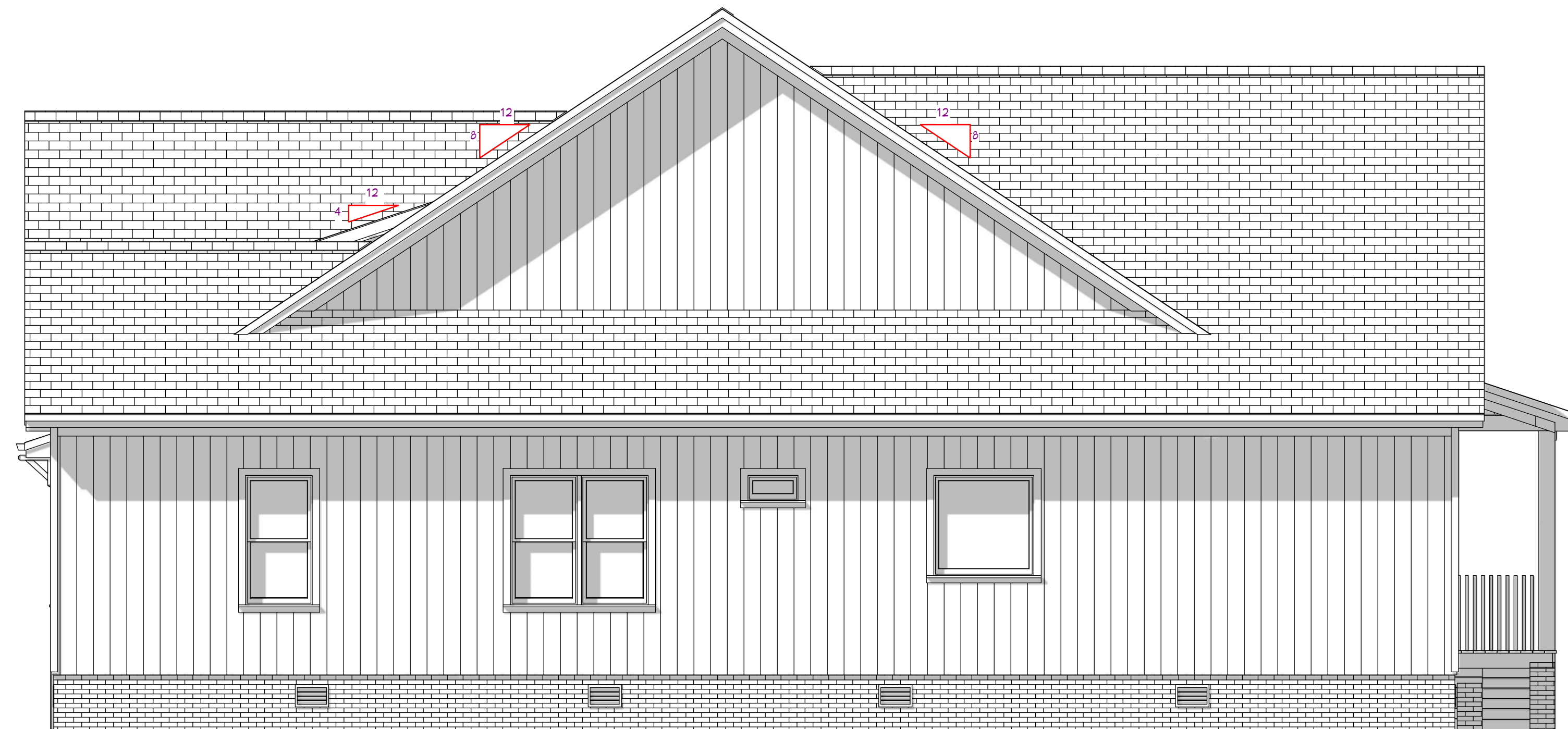
Exterior Elevation Right 1/4 in = 1 ft
