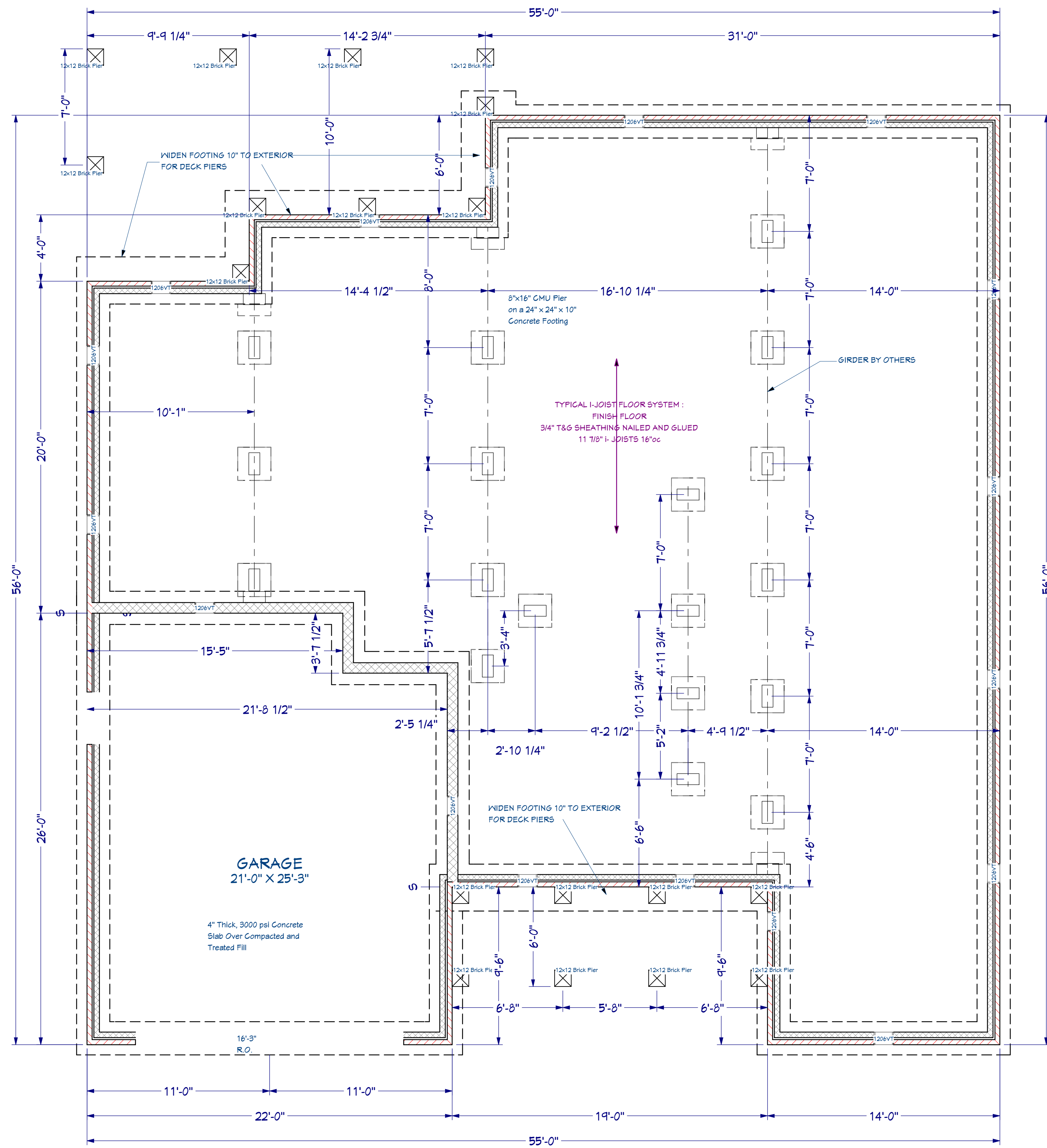
Working Plan View
