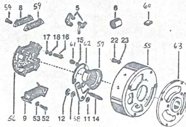
TYPE ● MAGNETO...with two ignition generating coils and one lighting coil.
