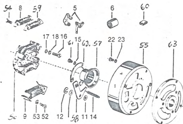
TYPE A MAGNETO... with two ignition generating coils and one lighting coil.
