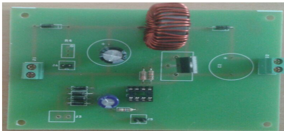
Fig. 10. SEPIC converter
