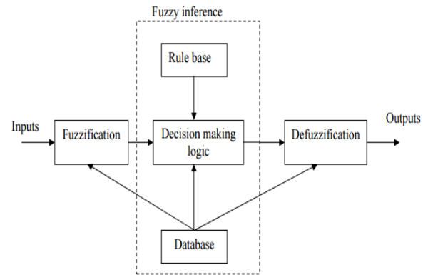
Fig. 4. Structure of Fuzzy logic controller
