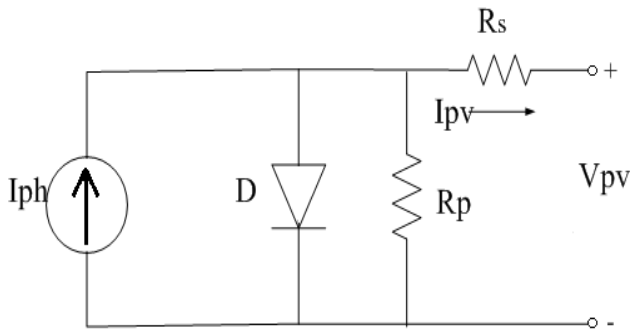
Fig. 3. Equivalent Circuit
