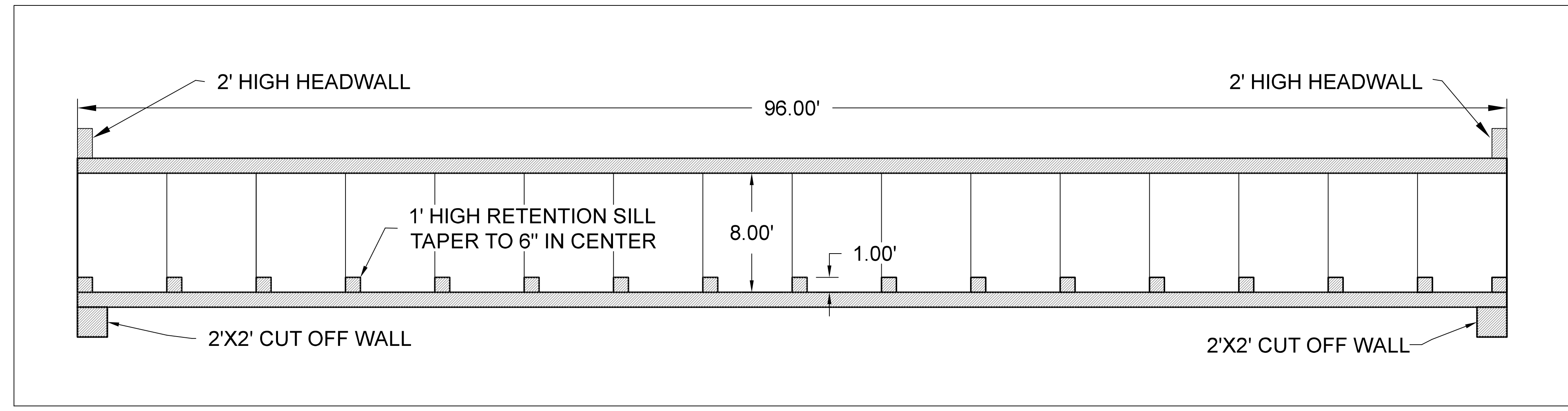
ELEVATION OF BOX CULVERT 1" = 5'
