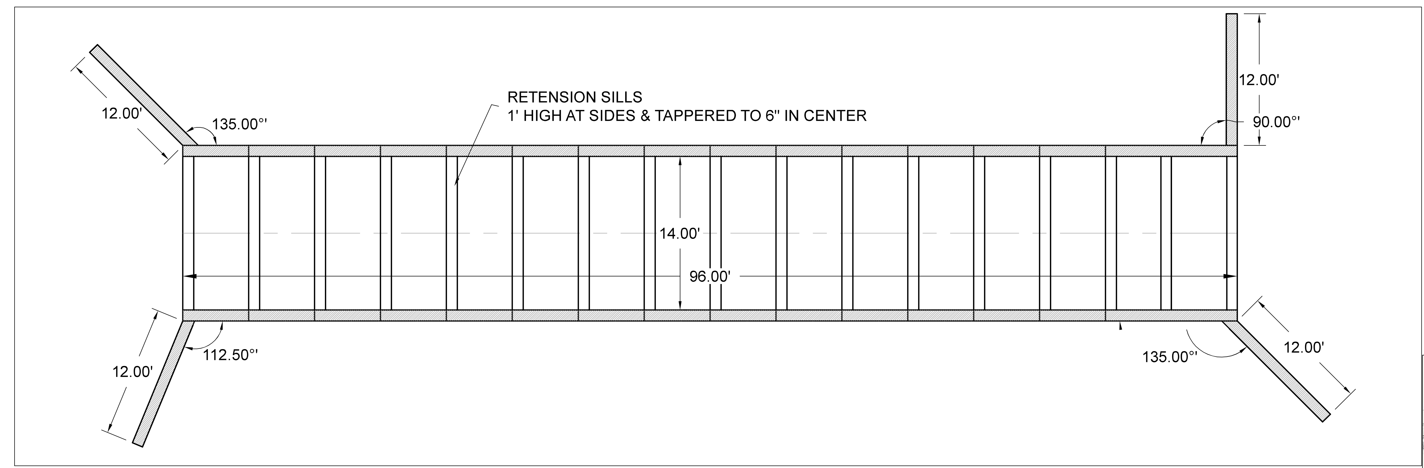
PLAN VIEW OF BOX CULVERT & WING WALLS 1" = 5'
