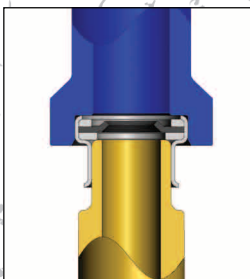
Seal Installation Detail
