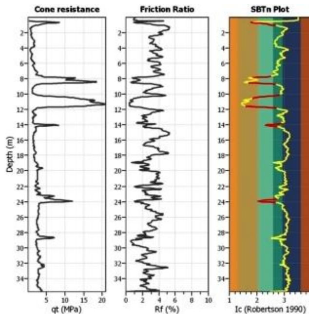
Figure 2. Typical CPT, California Site.
