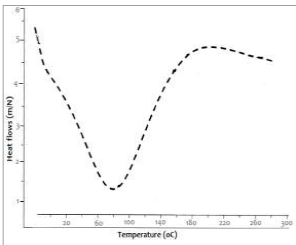
Figure 5. The DSC Curve of Pineapple Leaf Fiber
