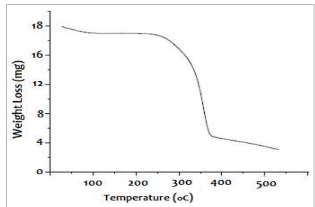
Figure 6. The TGA (Thermogravimetric analysis) Curve of Pineapple Leaf Fiber
