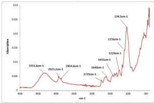
Figure 4. Result of pineapple fiber under FTIR
