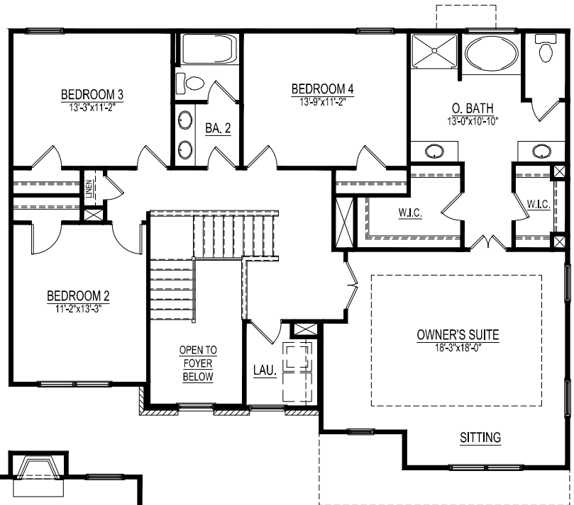
Second Floor
