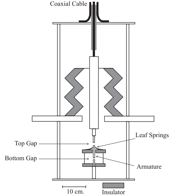
Fig. 2. Schematic description of the cylindrically symmetric experimental circuit, drawn to scale and showing only two of the six supporting legs.
