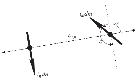
Fig. 5. Geometrical parameters used in Ampère's force formula, equation (12).
