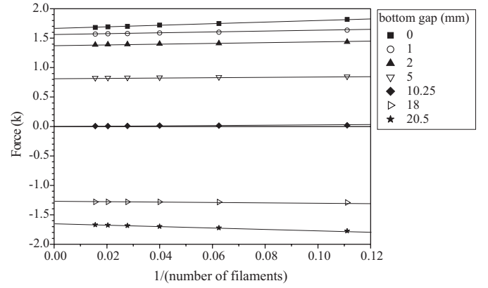
Fig. 7. Convergence calculation used to predict the Ampère force ( k ) for large numbers of filaments ( N ).
