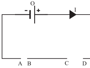
Fig. 1. Circuit used to demonstrate the importance of unequal air gaps in producing longitudinal motion.
