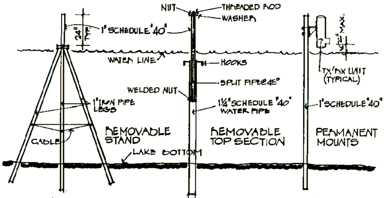
FIGURE 6 TRANSMITTER MOUNTS
