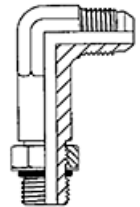
90° LONG STR. THREAD ELBOW 5503 (CC5OX-S)
