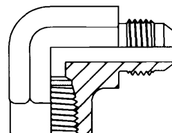
FEMALE 90° ELBOW 2203 (DTX)
