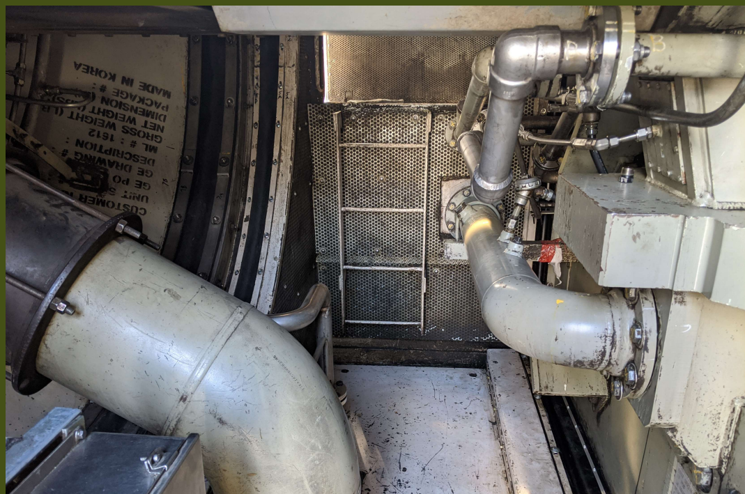
Load Compartment, Bellmouth, Turbine & Generator Enclosures - All Seals
