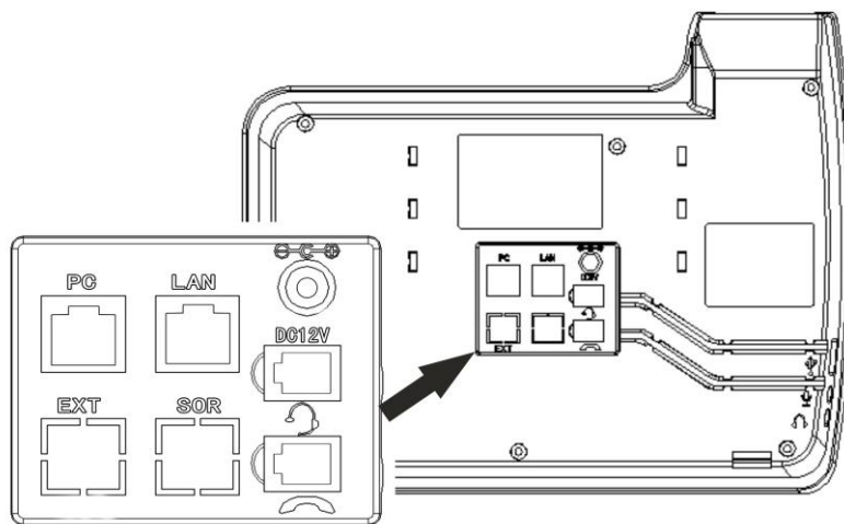
Figure 1 Connections on the back of IPitomy IP330
