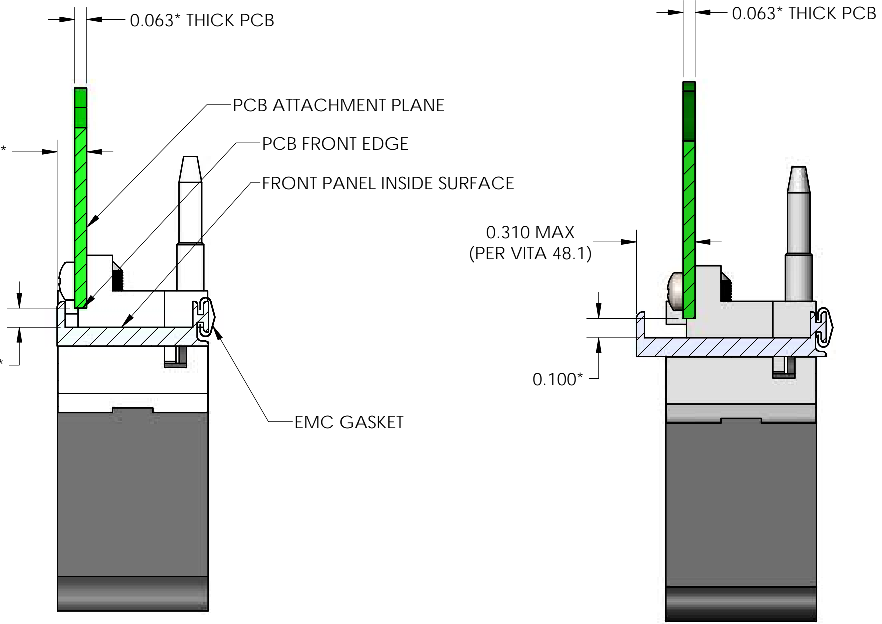
SECTION J-J FOR 3U, 6U, AND 9U 4HP, 8HP, 12HP WIDE PANELS. FRONT PLUG-IN CARDS. SCALE 2 : 1 SECTION E-E FOR 3U, 6U, AND 9U 5HP WIDE PANELS. FRONT PLUG-IN CARDS. SCALE 2 : 1
