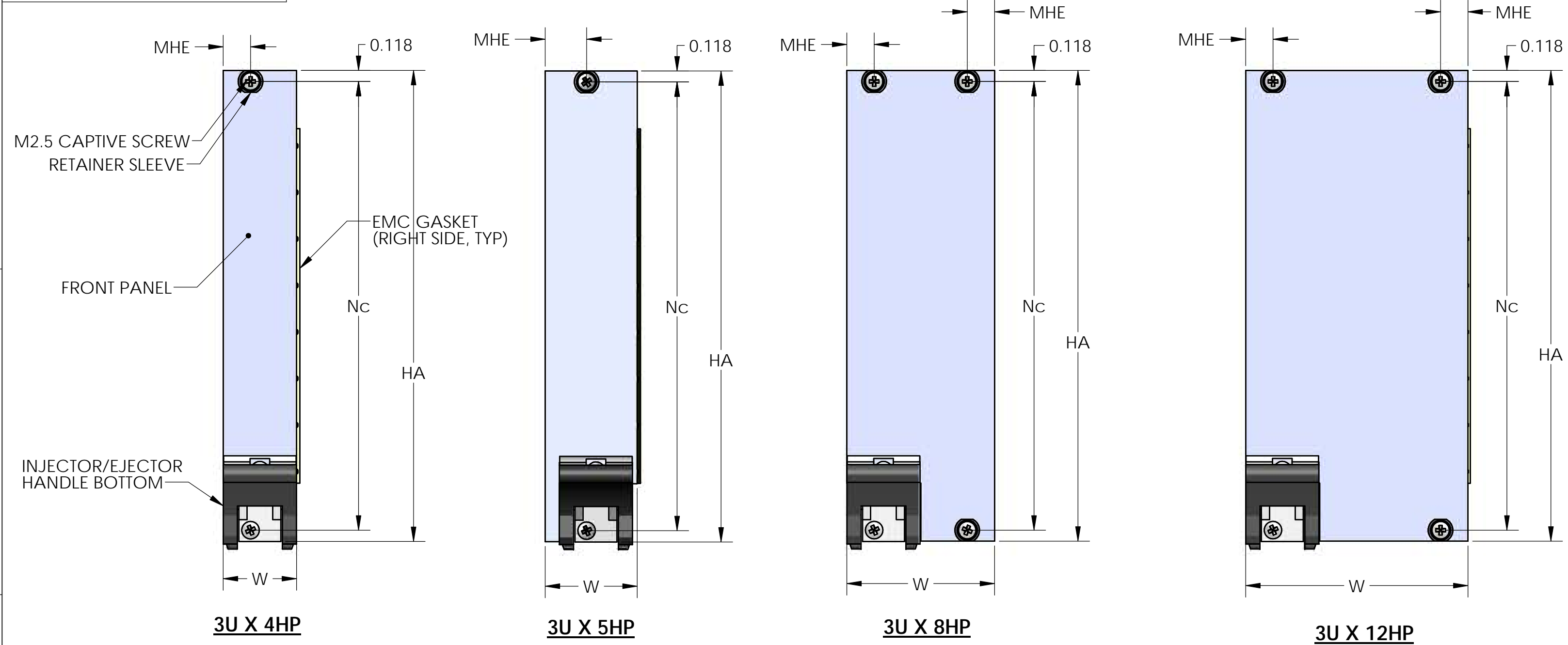
3U FRONT PLUG-IN CARDS, SEE SHEET 3 FOR 3U RTM (REAR TRANSITION MODULE)
