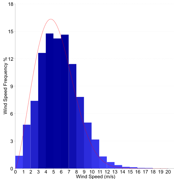
Figure 39: December speed frequency distribution at 30m hub height (bars).
