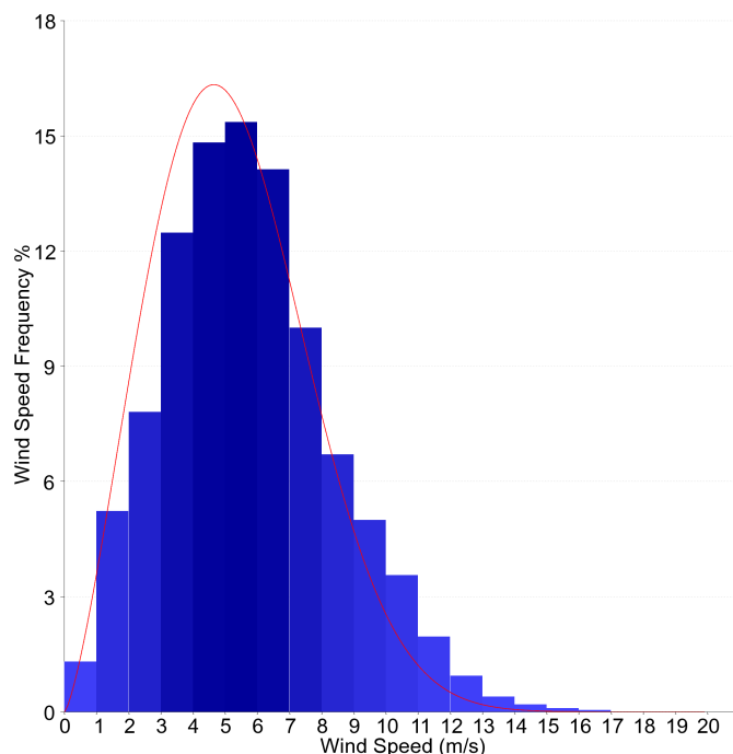
Figure 6: January speed frequency distribution at 30m hub height (bars).
