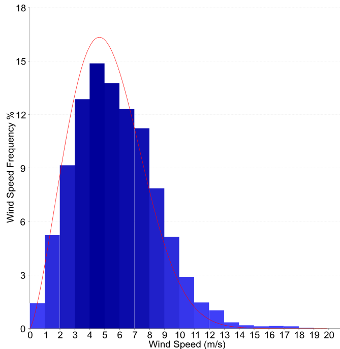
Figure 9: February speed frequency distribution at 30m hub height (bars).
