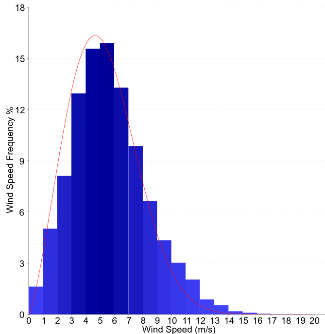
Figure 12: March speed frequency distribution at 30m hub height (bars).
