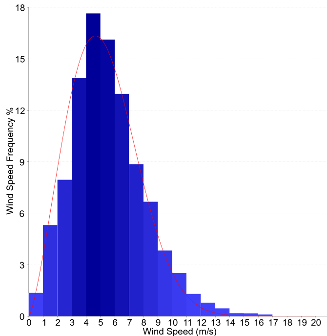
Figure 36: November speed frequency distribution at 30m hub height (bars).
