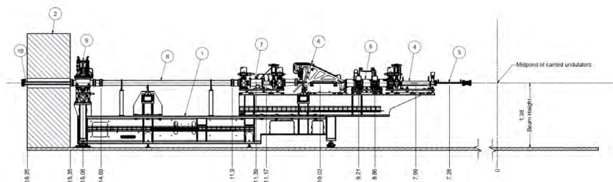
FIGURE 3: Layout of front end with beam direction right to left (numbered items are discussed in the text). Dimensions are in meters, rounded to the nearest centimeter.
