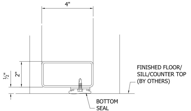
SECTION VIEW @ BOTTOM HORIZONTAL
