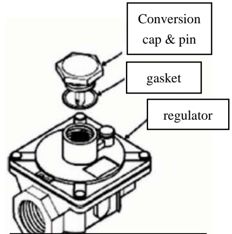
Fig.1 Gas pressure regulator
