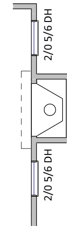
2 Fireplace w/ Window Opt. A-2.10 3/16" = 1'-0" WHEN PRINTED ON 11"x17" / ANSI B PAPER SIZE
