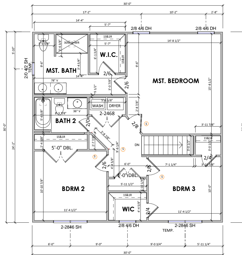
1 Second Floor Plan A-2.20 1/8" = 1'-0" WHEN PRINTED ON 11"x17" / ANSI B PAPER SIZE
