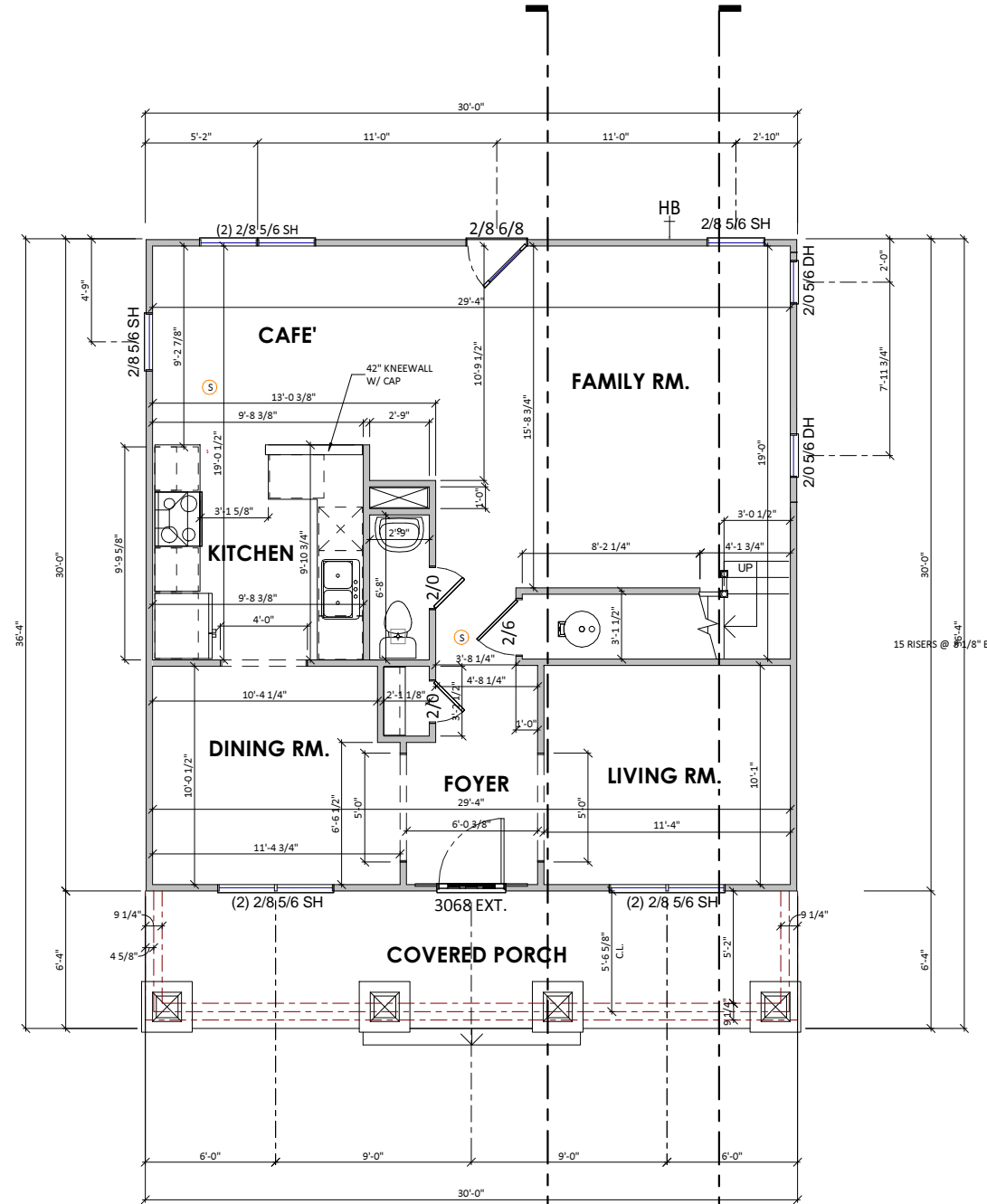
1 First Floor Plan A-2.10 1/8" = 1'-0" WHEN PRINTED ON 11"x17" / ANSI B PAPER SIZE
